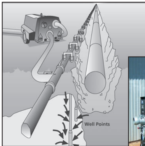
Sewer Bypass Well Point Dewatering Location Dewatering
